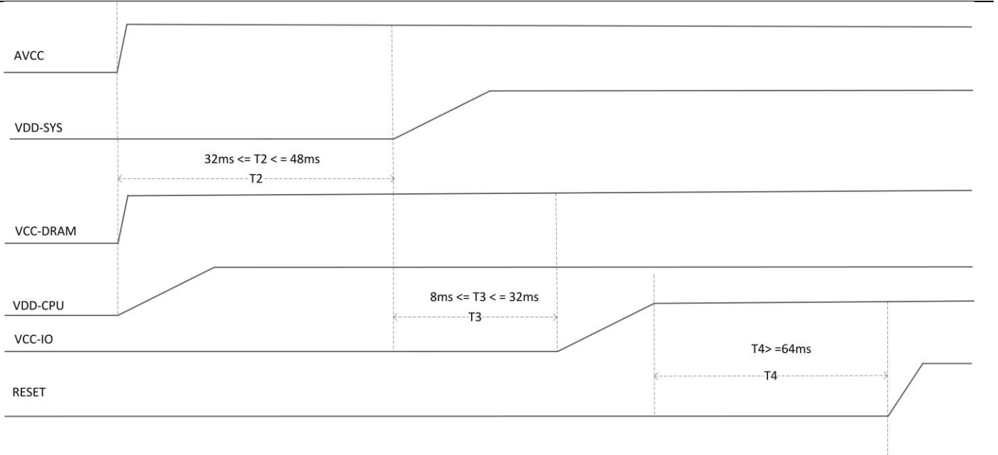
Figure 5.2: Power Up Reset Sequence
