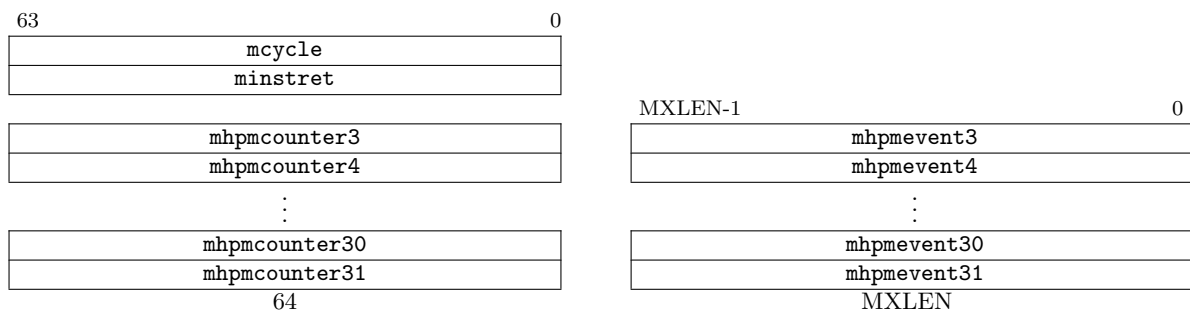
Figure 3.19: Hardware performance monitor counters.
