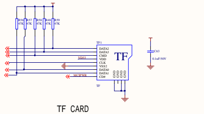
TF CARD
