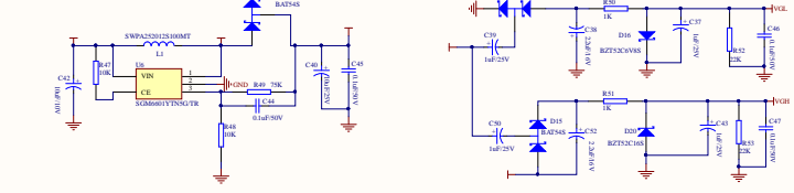
5V ->AVDD
