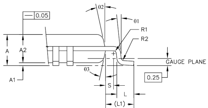
DETAIL F
