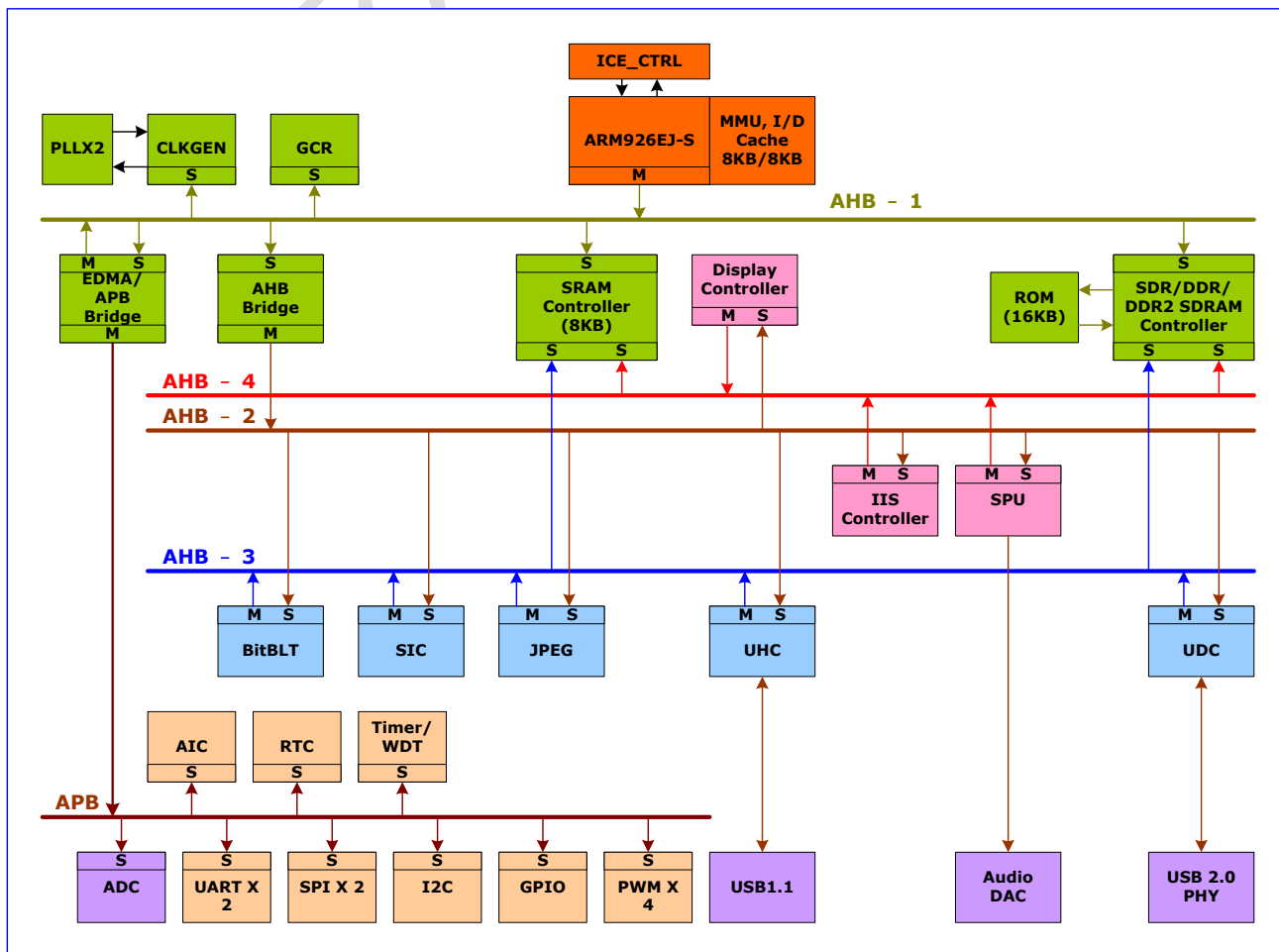
Figure 4.1 N9H20 Series Block Diagram
