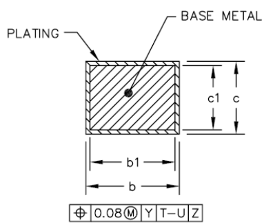
SECTION G-G
