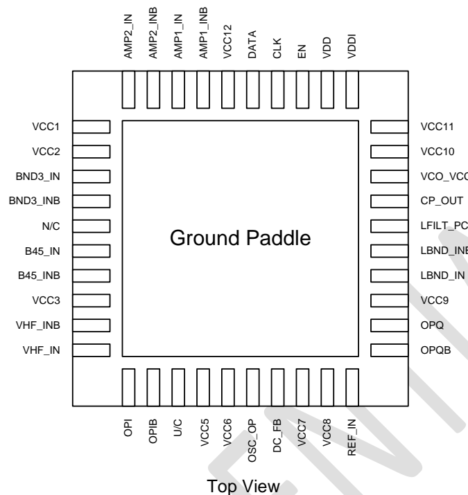
Figure 3: Pin-Out Diagram
