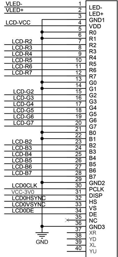
FPC40PIN-0.5
