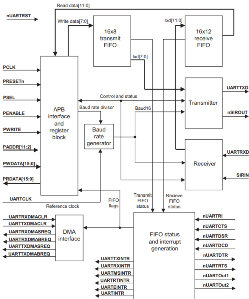
UART block diagram
